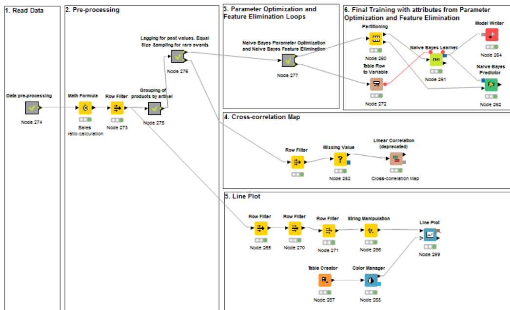
Fig. 6. Knime workflow. Stages of Model Training, Optimization and Testing
