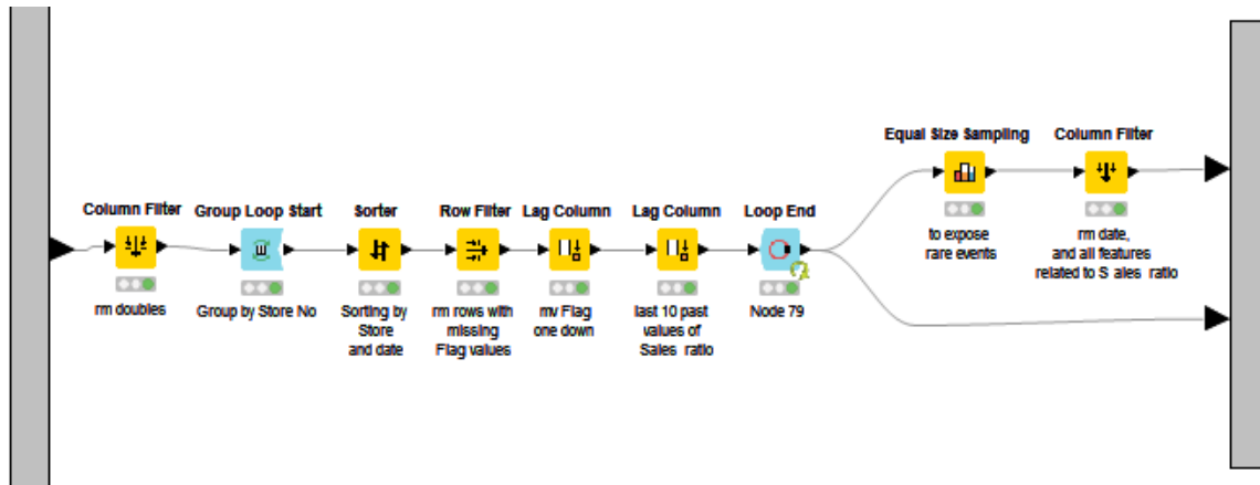
Fig. 9. Past values building metanode
