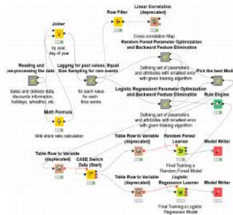
Figure 2. Demand prediction and replenishment models (top level of KNIME workflow)
