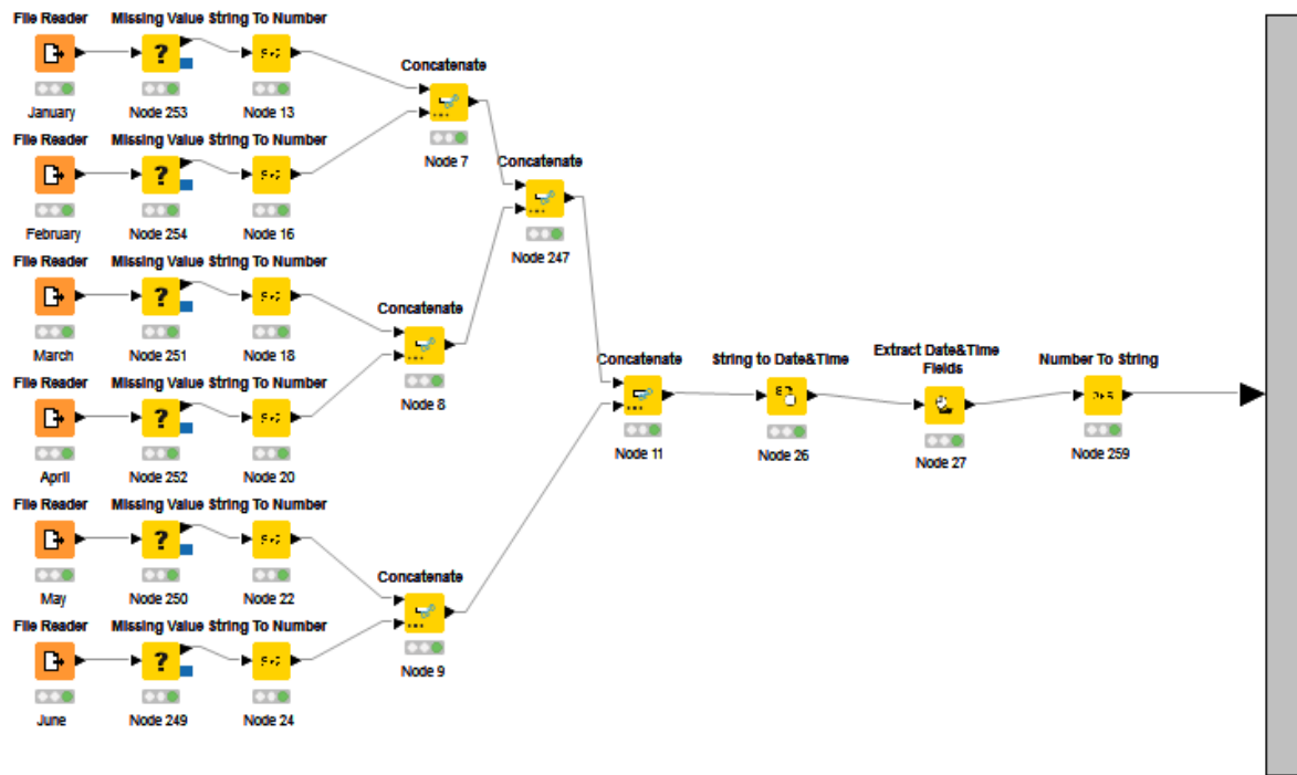
Fig. 7. Data reading and pre-processing metanode
