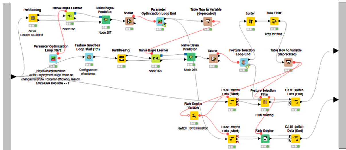
Fig. 11. Bayesian Parameter Optimization and Backforward Feature Elimination
