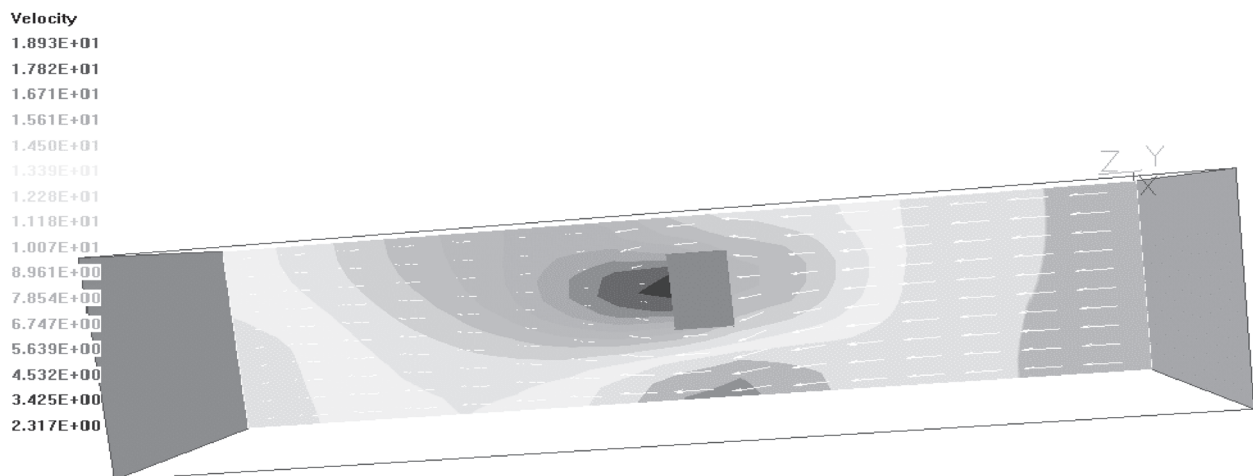
Fig 7. Decrease of velocity due to protective walls (velocity = 15 m/s)
