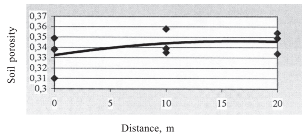
Fig 6. Change of soil porosity in tank field
