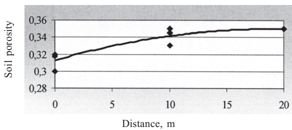
Fig 4. Dependence of soil porosity on distance to tracked vehicle route
