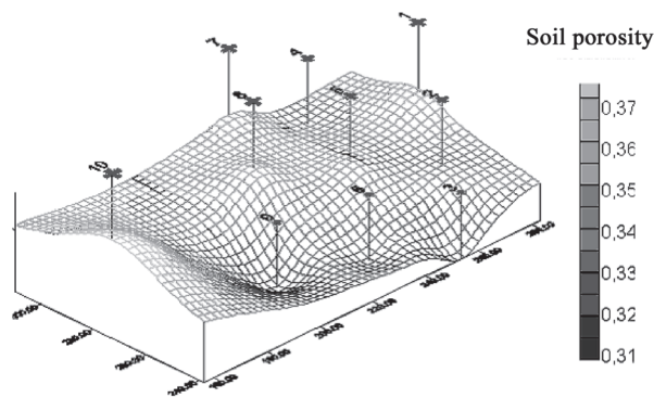
Fig 3. Distribution of soil porosity rate in tracked vehicle route
