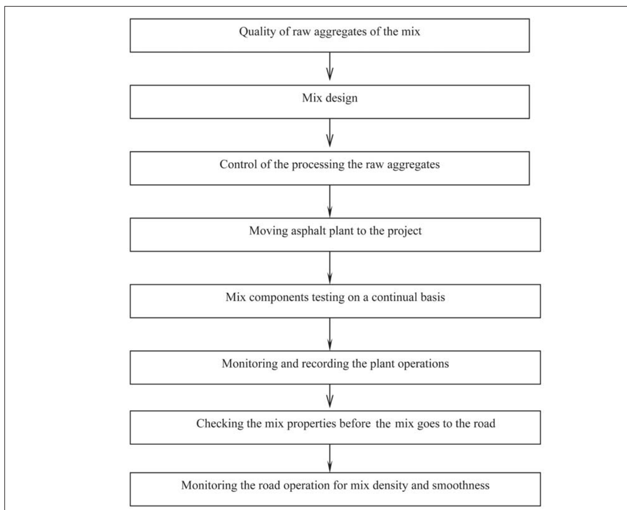
Fig 2. Asphalt concrete mix quality assurance system
