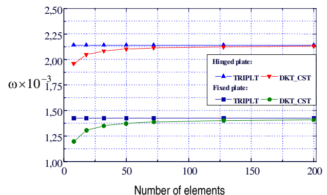
Fig 2. Convergence of values
