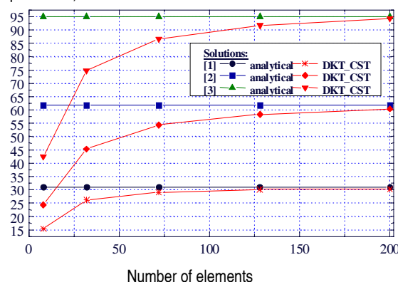
Fig 4. Convergence of the first three non-zero frequencies
