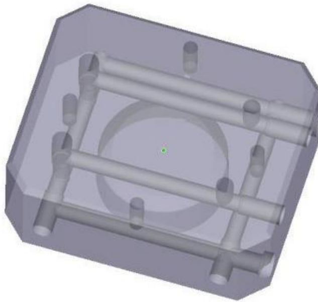
Fig. 6. Conventional channels [7]
