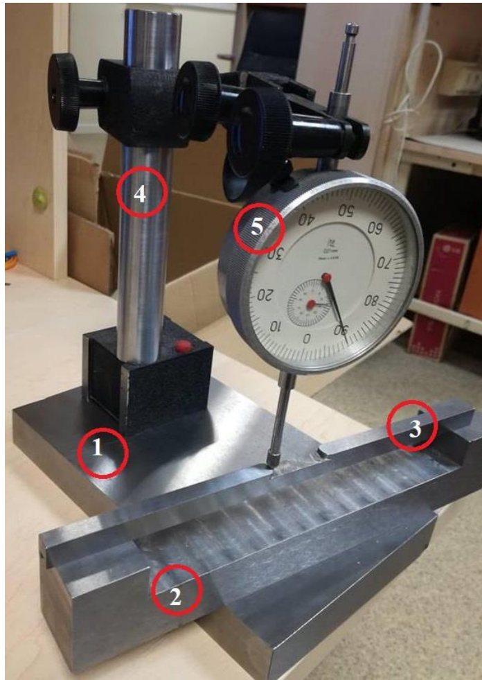
Fig. 20. Measuring system for points 5 and 6
