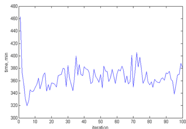
Figure 2 (b). ACO computational results using more than 17 ants (2 nd production line)
