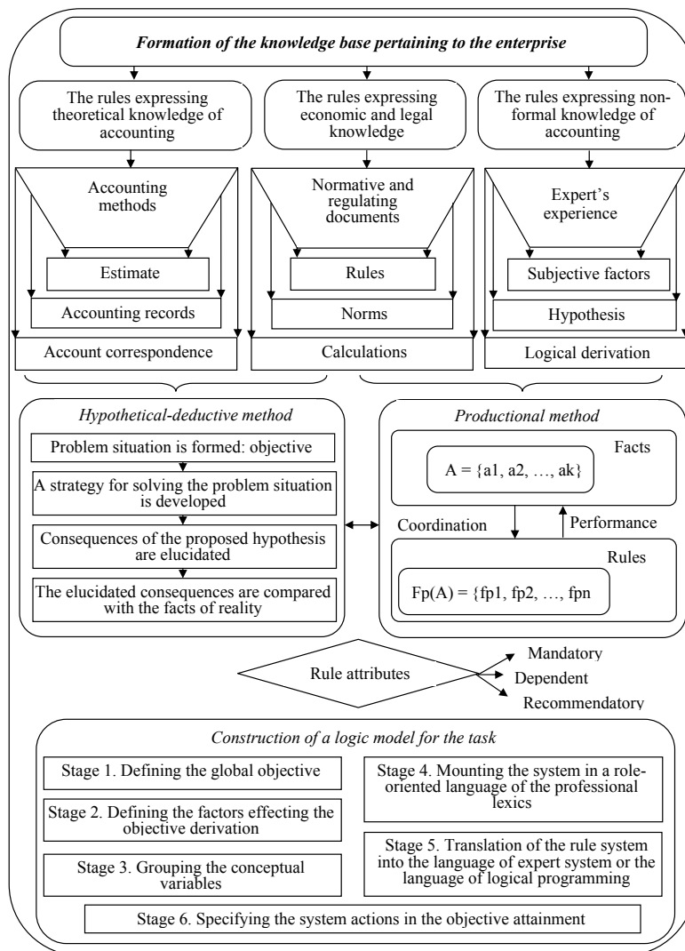
Fig. 1. The model of construction of the knowledge base during formation of the enterprise accounting policy in an intelligent accounting system
