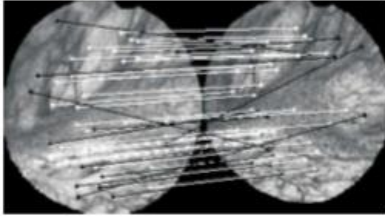
Figure 3 Rejected outlier points (labeled black) performed by the RANSAC algorithm [3]
