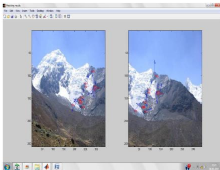
Figure 1 Keypoint detection [1]
