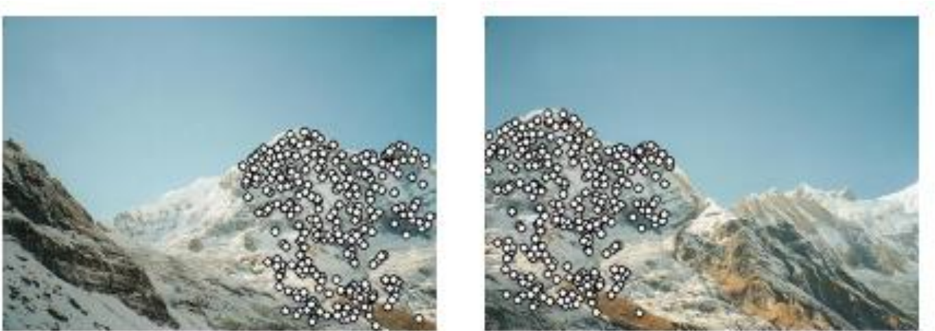
Figure 12 SIFT matches [9]
