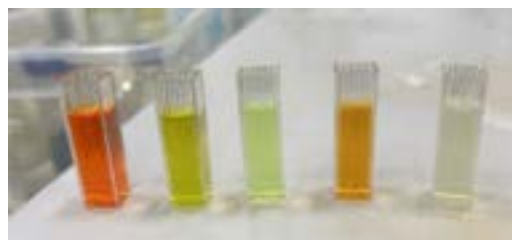
Figure 1. Brooker's Merocyanine complexes with metal solutions. From left to right: 0,1 mmol/l Brooker's Merocyanine solution; 0,1 mmol/l \text{Ni}^{2+} , \text{Cu}^{2+} , \text{Co}^{2+} , \text{Al}^{3+} solutions combined with dye 1:1 ratio.
