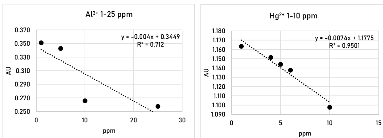
Figure 2. Calibration curve for the calculation of \text{Al}^{3+} and \text{Hg}^{2+} ion concentration in plants.
