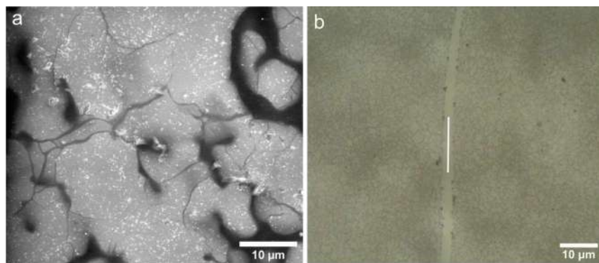
Fig. 1. PVB-Cu NPs coating. (a) Typical scanning electron microscope micrograph. (b) Optical microscope micrograph of the coating after mechanical resistance testing with 5 N load.
