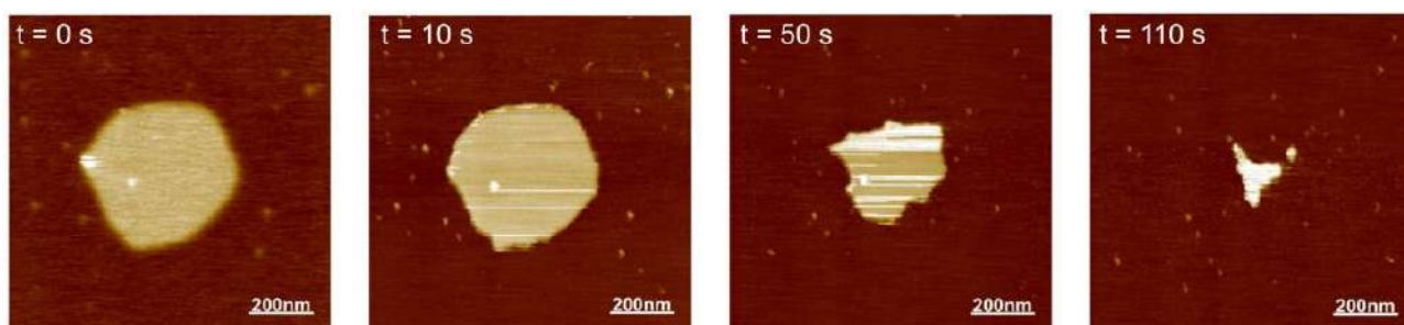
Fig. 1. High-speed atomic force microscopy images of S100A8-induced membrane dissolution. At the initial time point ( t = 0 s), the protein was injected into the fluid cell. The interaction between S100A8 and the negatively charged membrane leads to a detergent-like effect.
