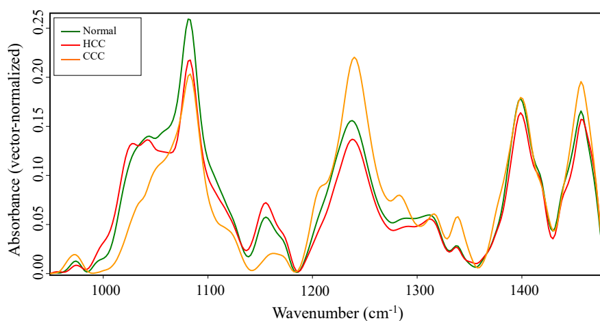
Fig. 1. Mean ATR IR spectra of liver normal and primary tumor (hepatocellular carcinoma (HCC) and cholangiocarcinoma (CCC)) tissue.
