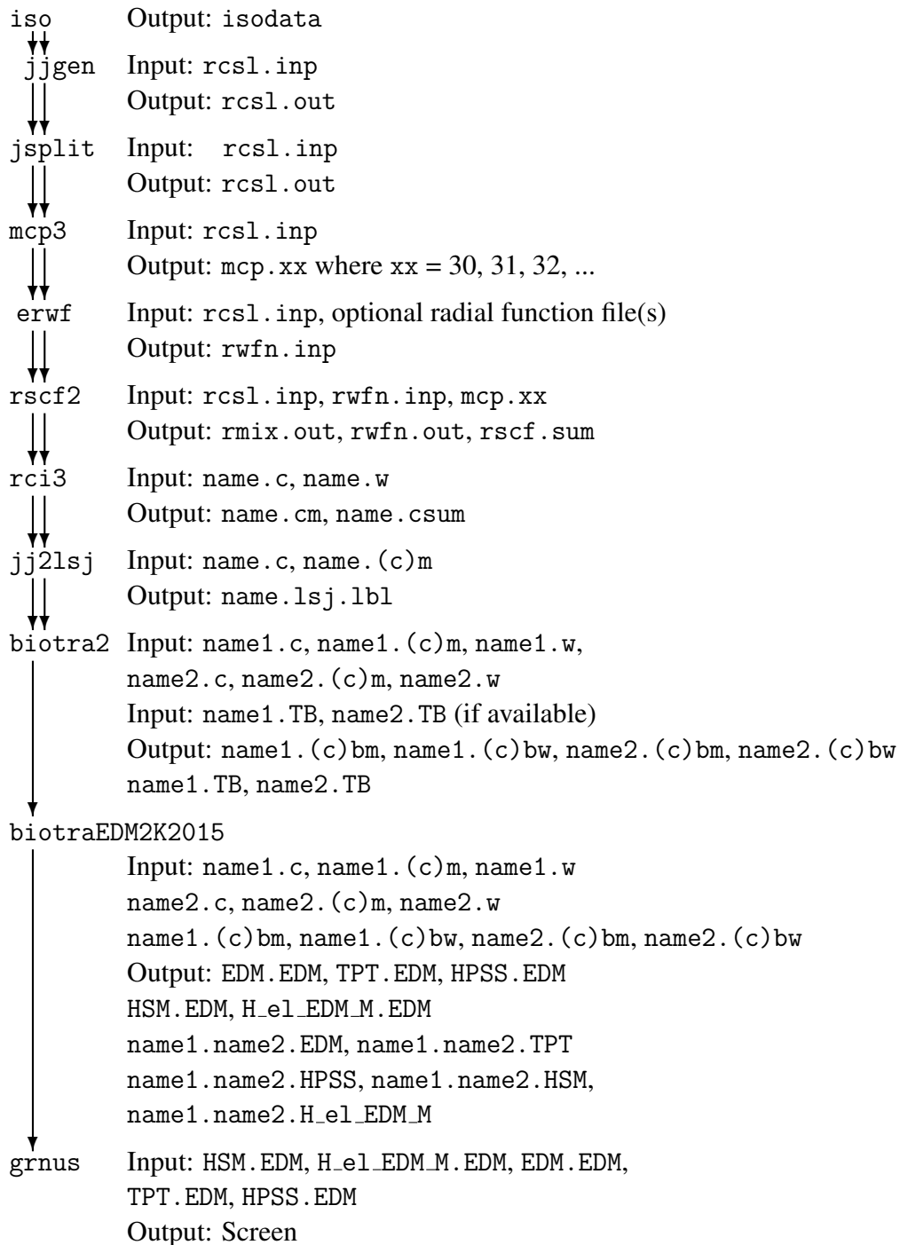
Figure 2.4.1: Flow of files for a normal sequence of program runs.
