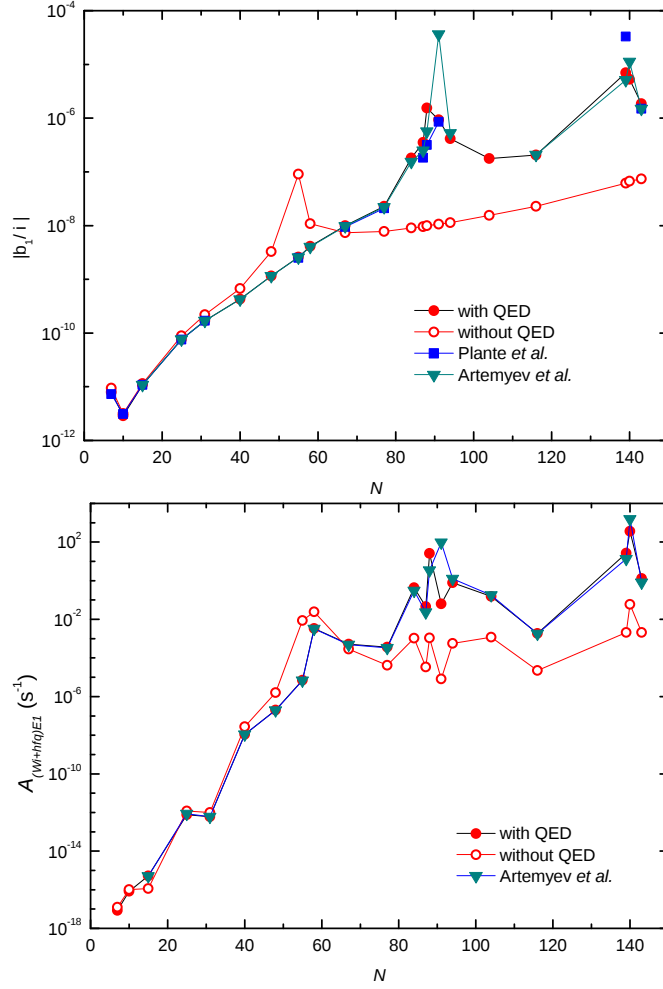
Figure 5.2.2: Dependence of mixing coefficient b_1/i (absolute value) and transition rates A_{(Wi+hfq)E1} on number of neutrons ( N ). The results calculated using energies from references Plante et al. [131] (squares) and Artemyev et al [132] (triangles) are also presented.
