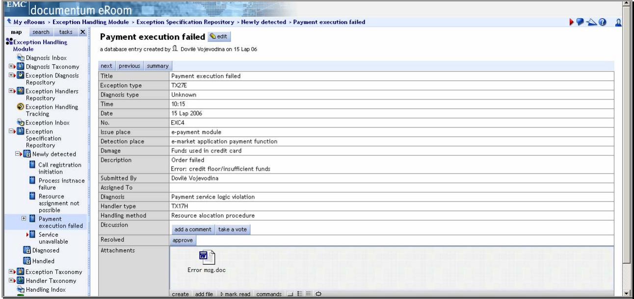
Picture 72. Exception repository record, containing full description of attributes and descriptive information in attachment box.
