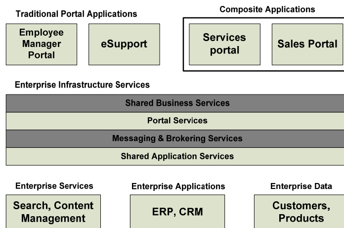
Picture 47. High level SOA solution model [7].
