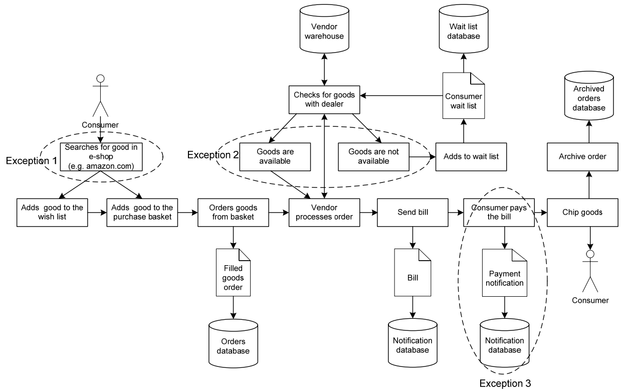
Picture 8. Purchase order workflow.
