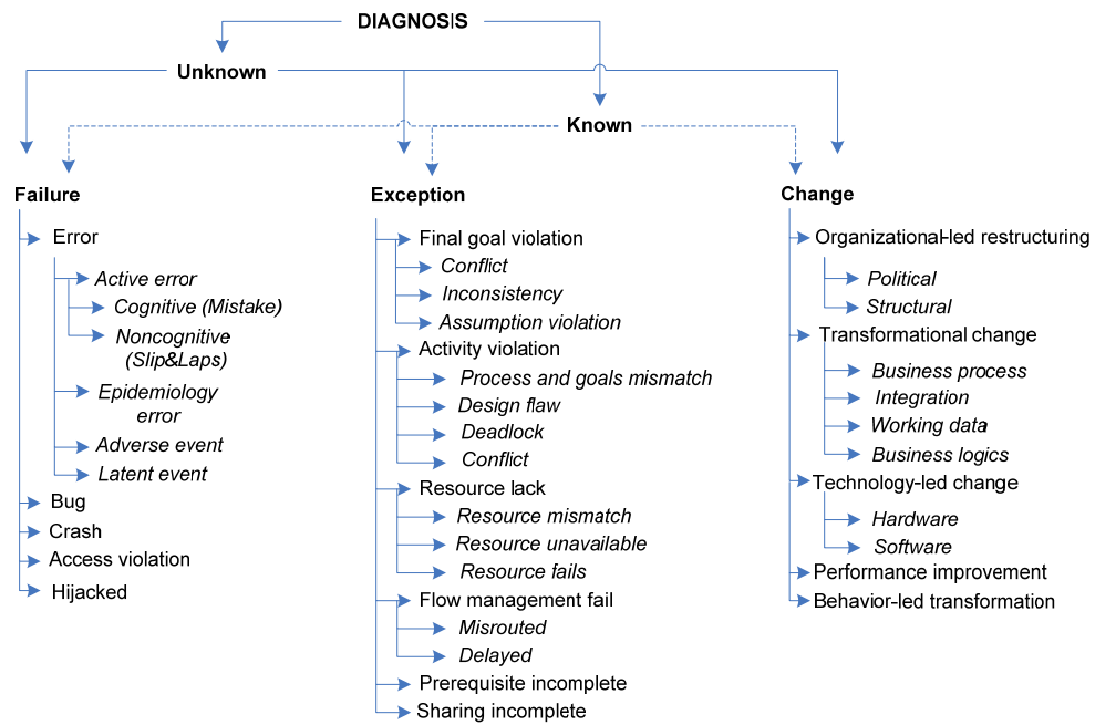
Picture 56. Diagnosis taxonomy, containing failure, exception and change types.
