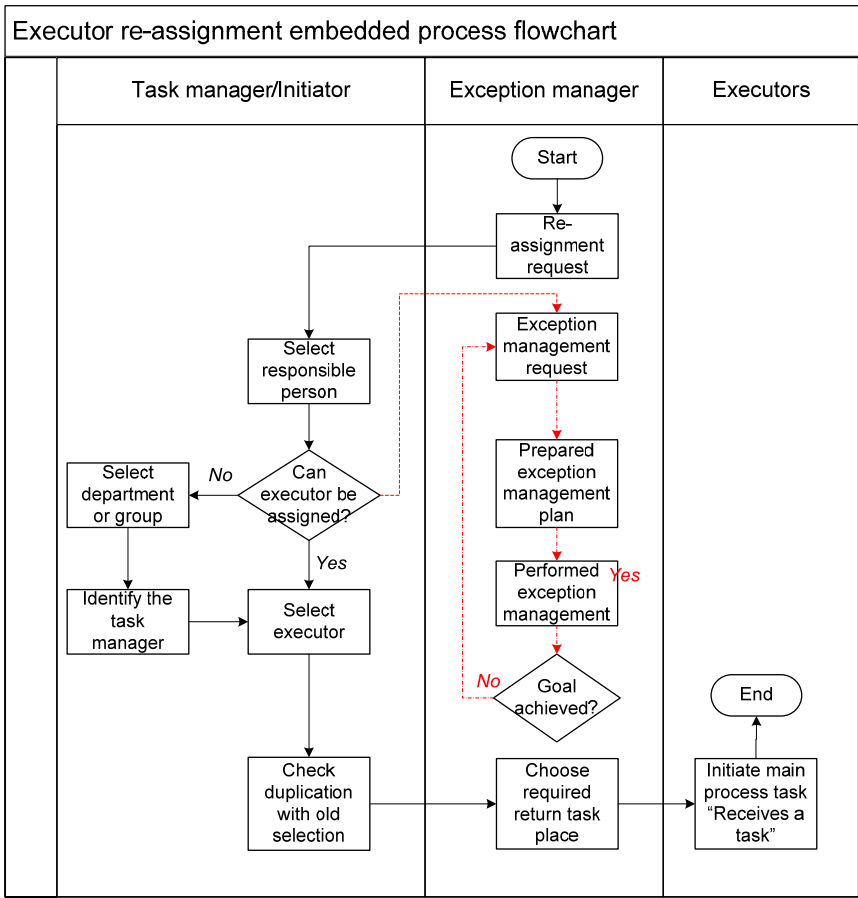
Picture 36. Executor re-assignment embedded process flowchart.
