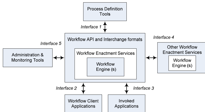
Picture 22. WfMC Reference Model [21, 80].
