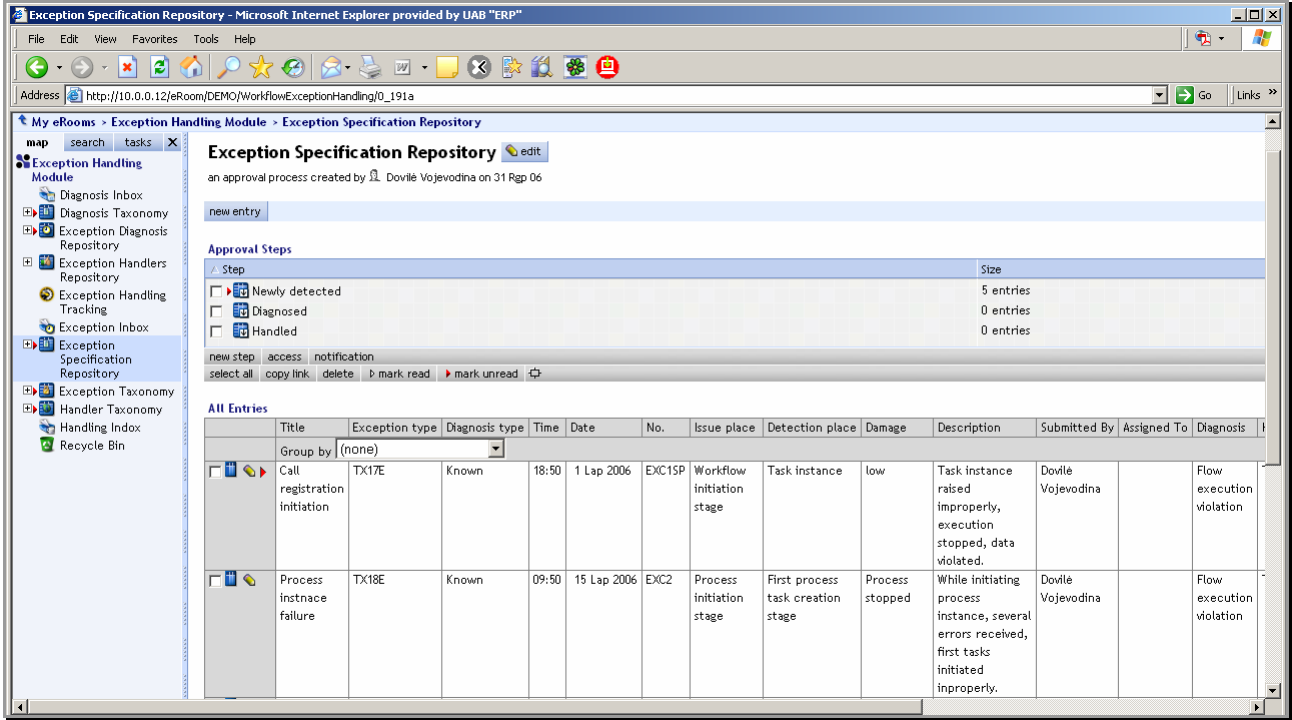
Picture 71. Exception specification repository with main lifecycle steps and collected records.
