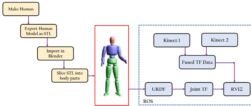
Fig. 10. Process of creating a human model for visualization in RViz.
