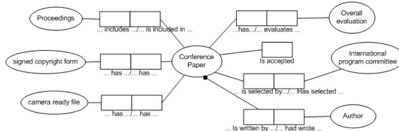
Figure 4.12. Source ORM Conference model
