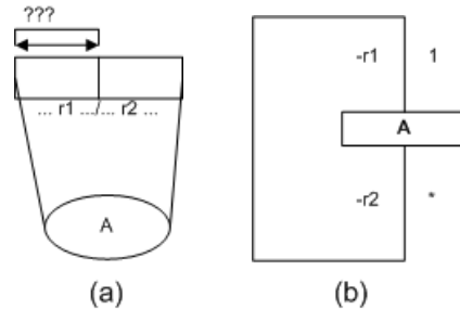
Figure 4.9. (a) Role with undefined ring constraint, (b) resulting UML model
