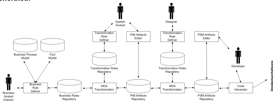
Figure I.1. Business rules transformation schematically
