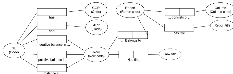
Figure 5.2. Domain ORM model
