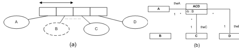
Figure 4.5. (a) N-ary role internal uniqueness constraint, (b) resulting UML model
