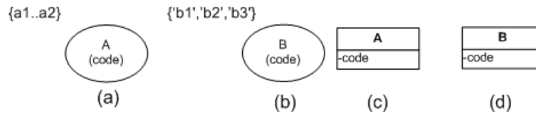
Figure 4.8. Entity type with (a) value range constraint and (b) value list constraint, (c,d) resulting UML model
