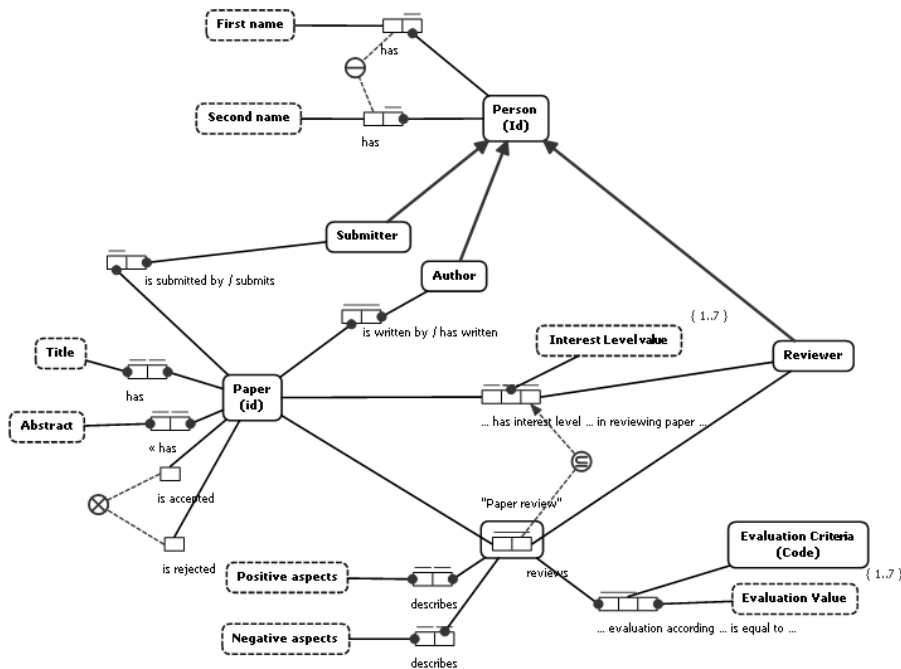
Figure 4.10. Source ORM model for the transformation example
