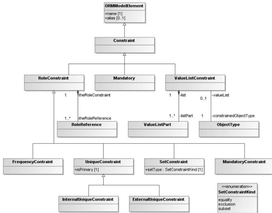
Figure 3.4. Constraints of ORM metamodel
