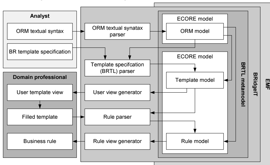
Figure 3.8. BRidgeIT tool architecture
