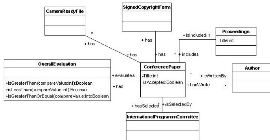
Figure 4.13. Resulting UML model of Conference domain
