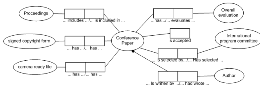
Figure 3.7. ORM Conference model
