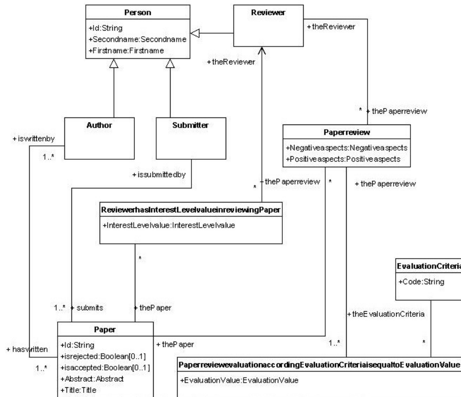
Figure 4.11. Example of resulting UML model
