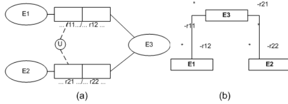
Figure 4.6. (a) External uniqueness constraint on the binary fact type, (b) resulting UML model
