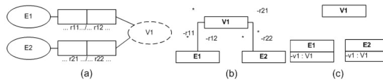
Figure 4.1. (a) Value type of source ORM model can be transformed to several types of UML class diagrams (b, c)
