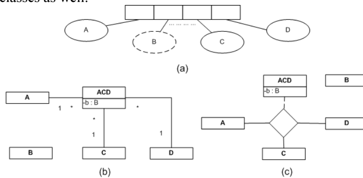
Figure 4.2. Transformation of n -ary fact (a) type to combination of association and class (b) and to UML ternary association (c)
