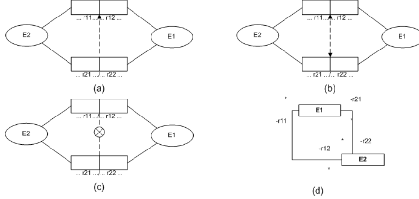
Figure 4.7. (a) subset, (b) equality, (c) exclusion constraint on binary fact type, (d) resulting UML model
