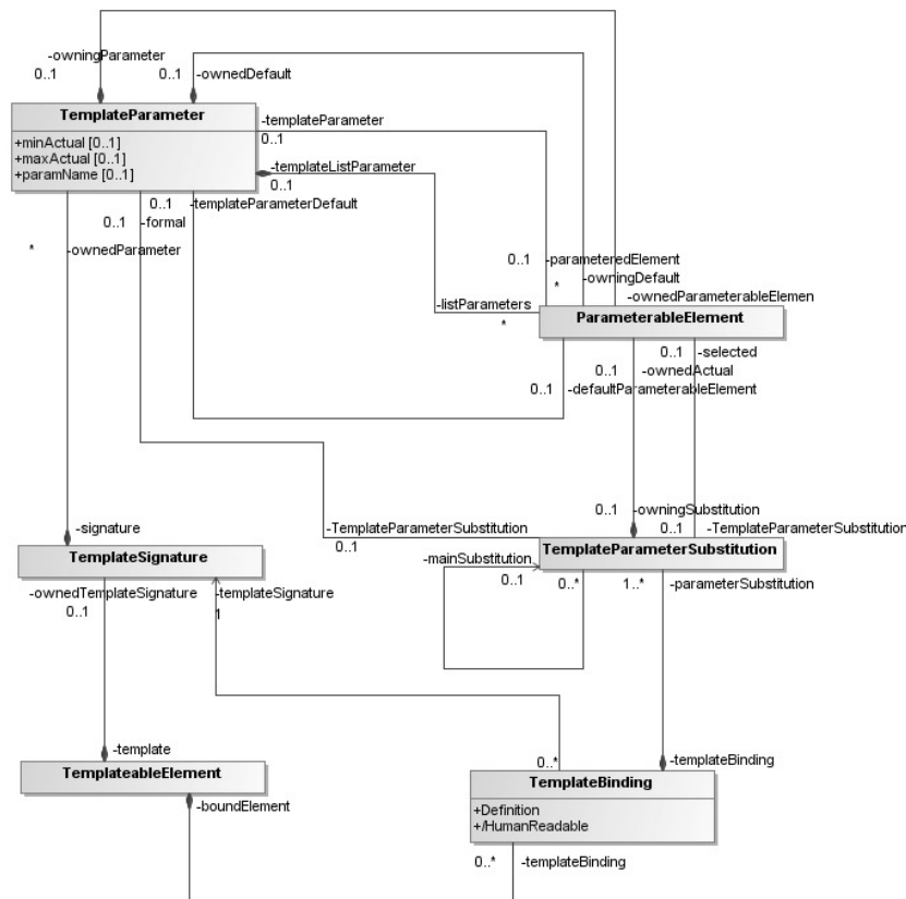
Figure 3.6. Template metamodel fragment
