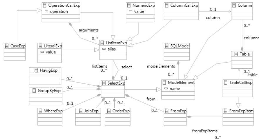
Figure 5.3. SQL select statements simplified metamodel
