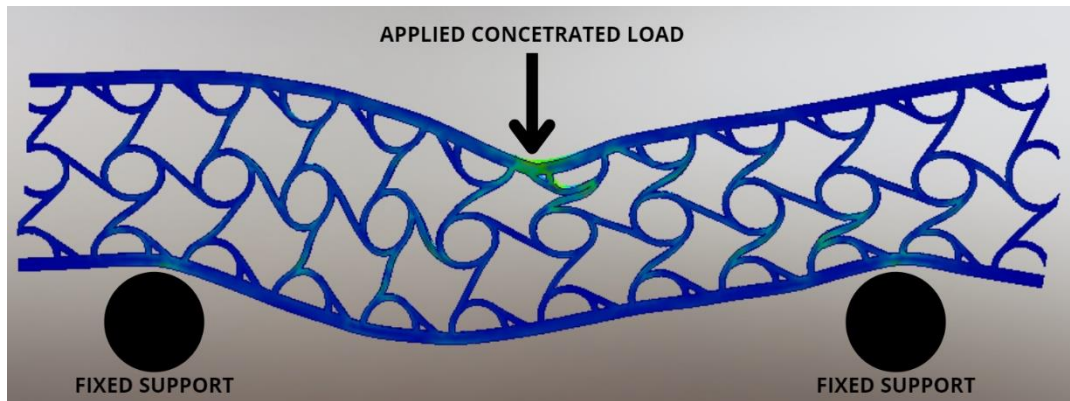
Fig. 3.12. Scheme of experiment in the Solidworks software.
