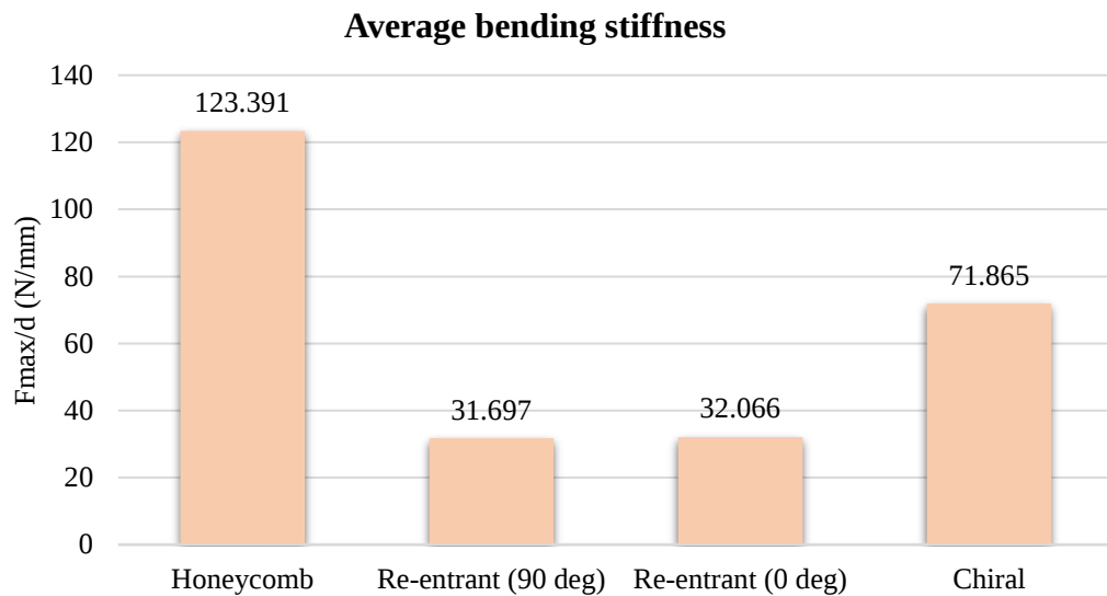
Fig. 3.3. Average bending stiffness
