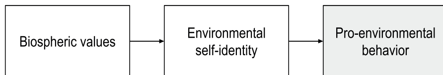
Figure 1 Theoretical Model on the Relationship Between Biospheric Values, Environmental Self-Identity and Pro-Environmental Behavior (adopted from van der Werff et al., 2014b)
