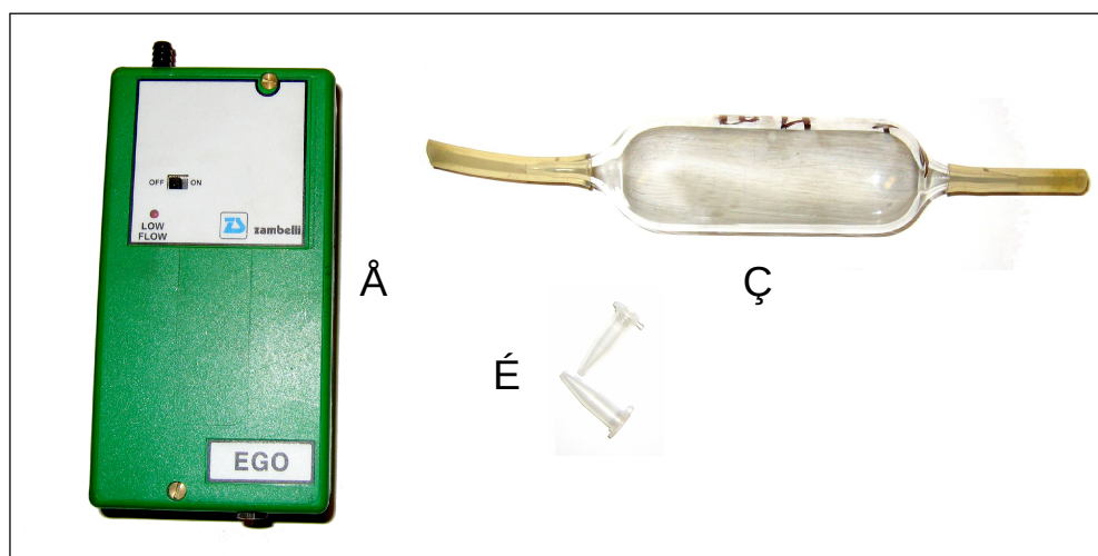
Figure 2.3. Sampling equipment: 1 – sampling pump, 2 - gas pipette, 3 – plugs.
