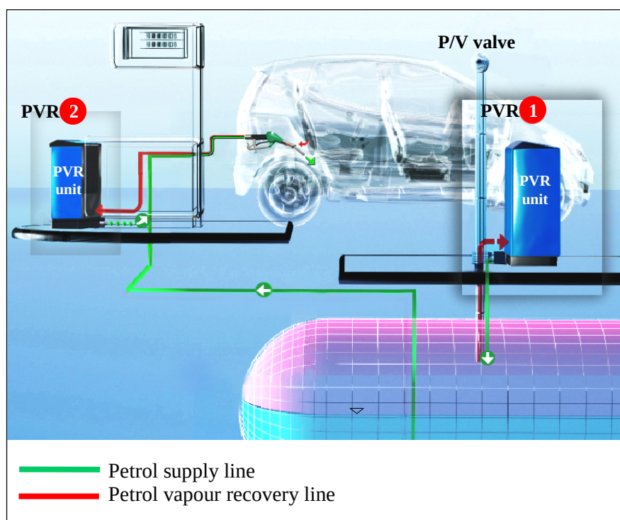
Figure 1.12. Vapour recovery system with refrigeration technique
