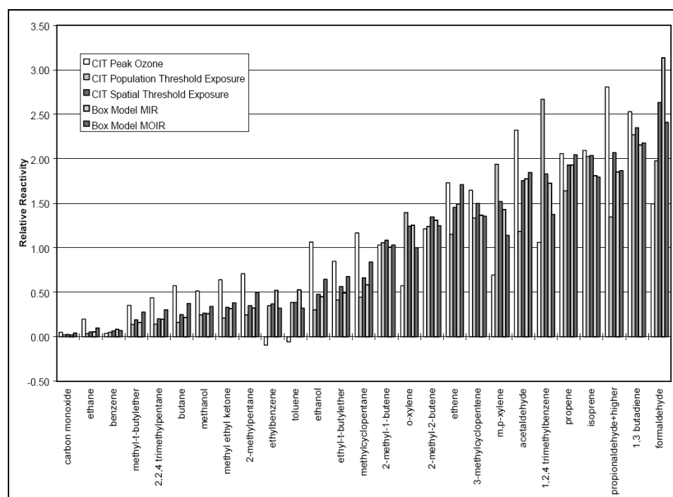
Figure 1.5. Modelled VOCs relative reactivity (VOC reactivity... 1999)
