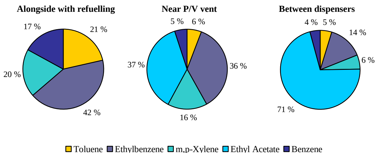
Figure 3.7. VOC composition in sampling points, Research site No. 1
