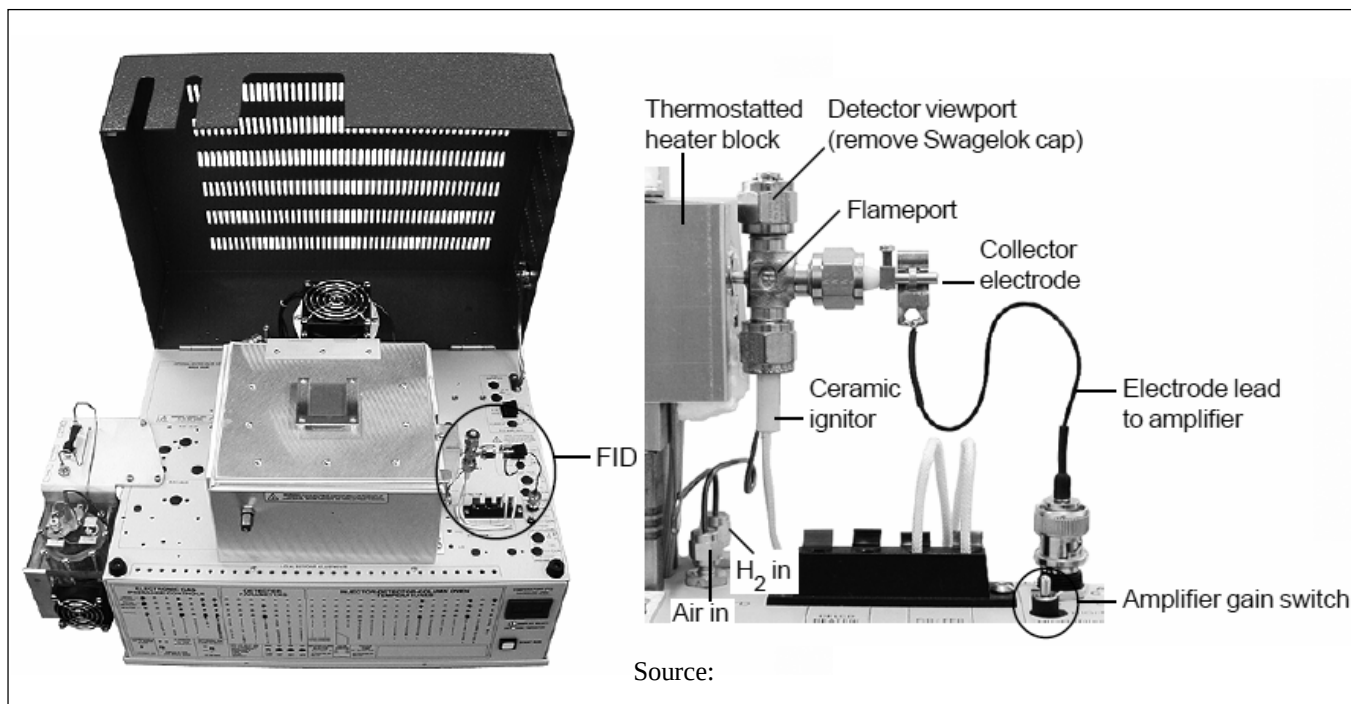
Figure 2.5. SRI capillary FID GC with built-in hydrogen generator
