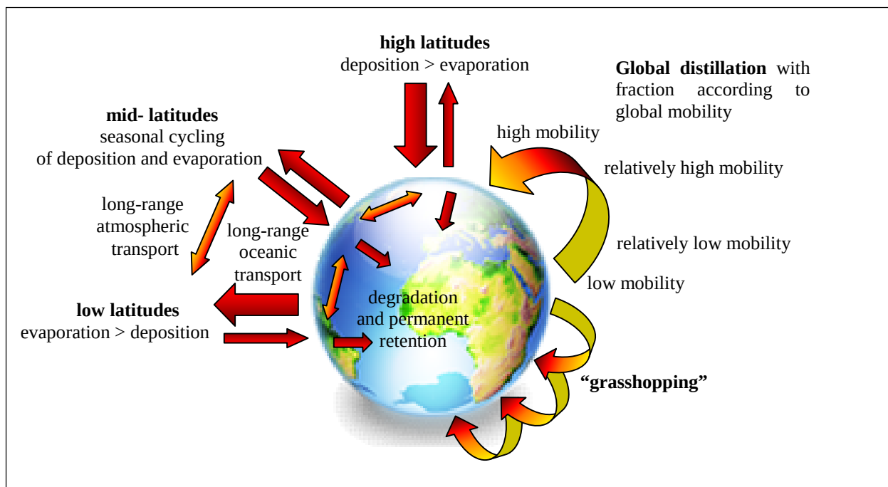
Figure 1.1. Migration of persistent organic pollutants in the global atmosphere
