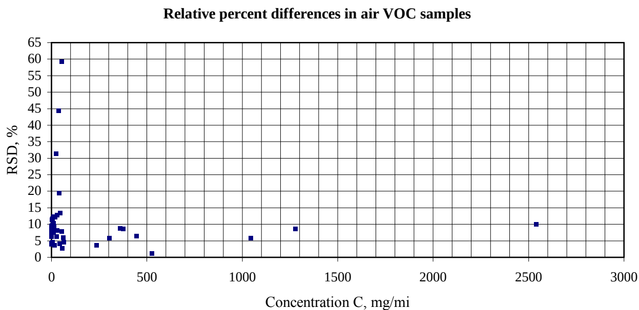
Figure 3.1. Relative percent differences in air VOC samples
