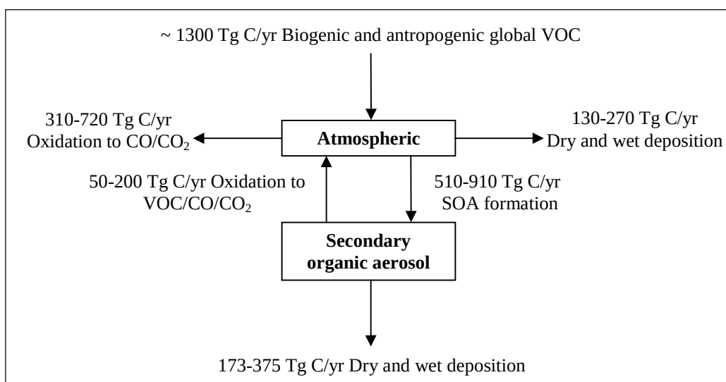
Figure 1.8. Mass-balance-based estimate of the global budget for atmospheric VOCs
