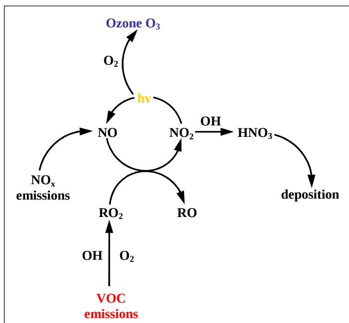
Figure 1.4. Schematic ozone photochemistry driven by VOCs
