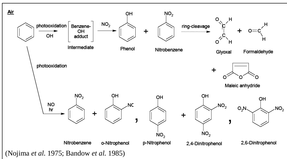
Figure 1.3. Environmental benzene transformation product in air
