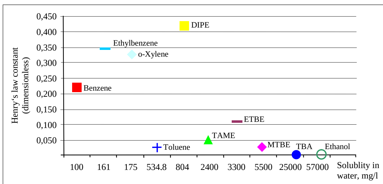
Figure 1.9. Relative solubility and Henry's law constants for selected VOCs and fuel oxygenates
