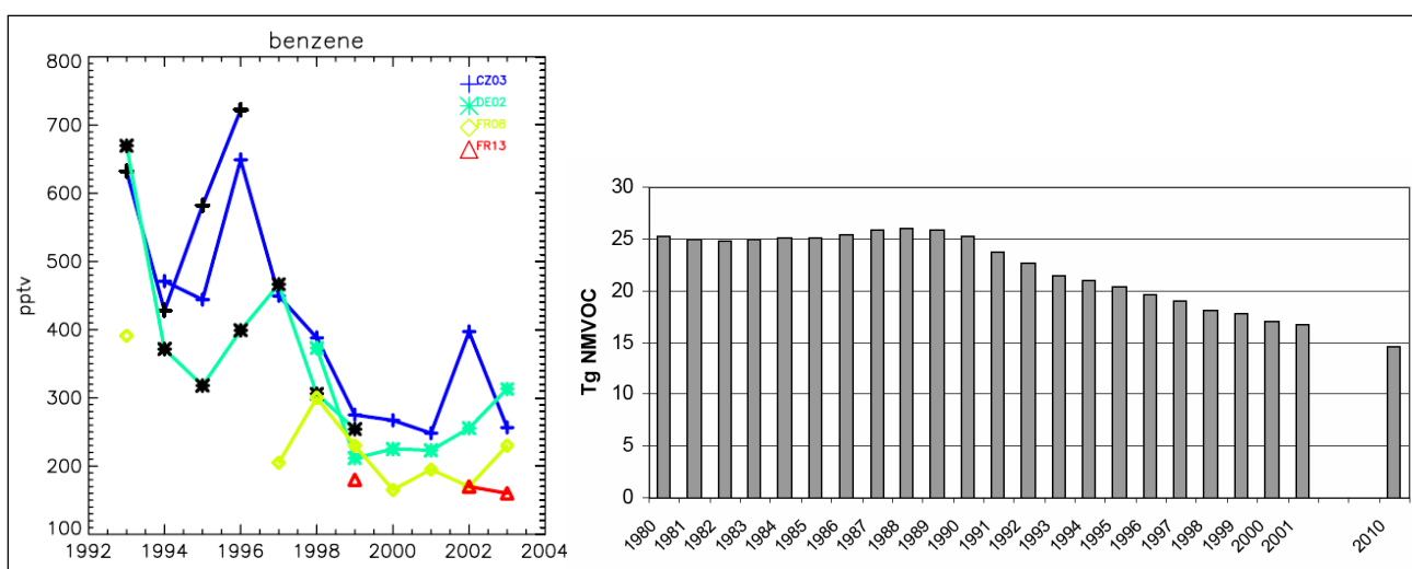
Figure 1.14. Benzene and NMVOC long-term trend in EMEP area (Solberg 2005)
