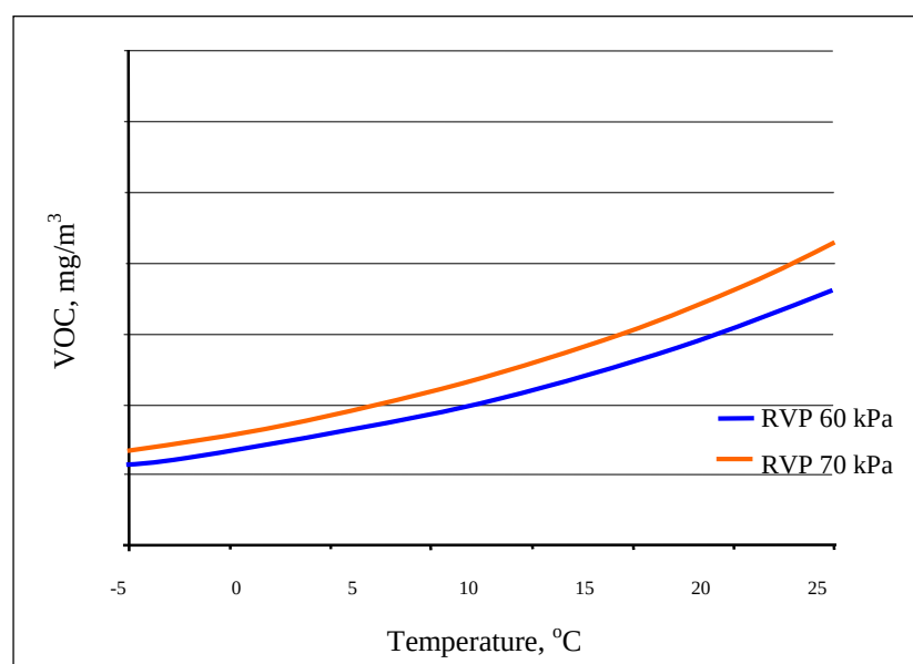
Figure 1.15. Petrol-related VOC emission dependence on ambient temperature
