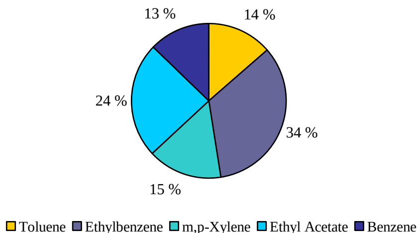
Figure 3.8. VOC composition in ambient air of petrol station, Research site No. 1
