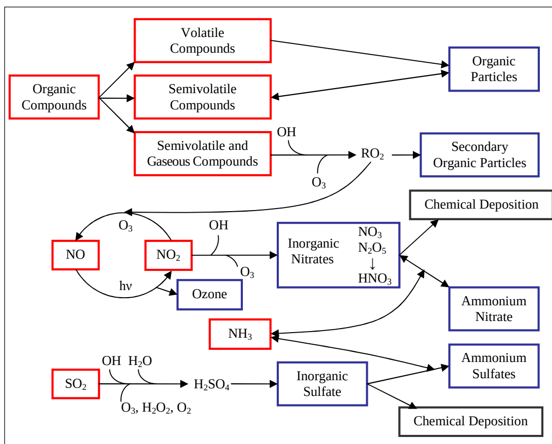
Figure 1.7. Chemical links between the VOC, ozone and PM formation processes
