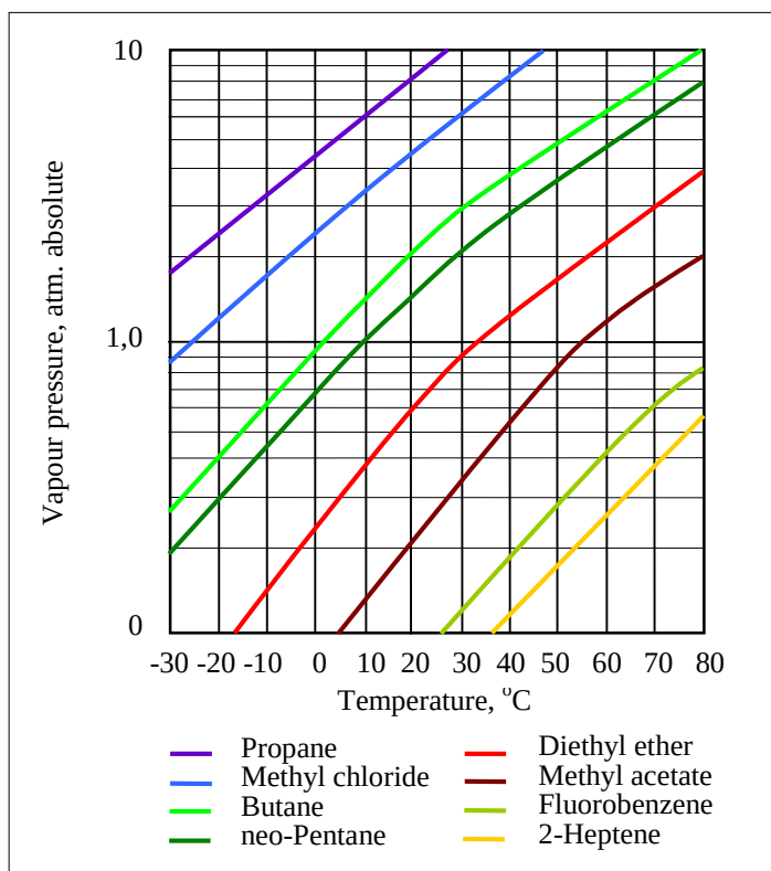
Figure 1.10. Vapour pressure chart
