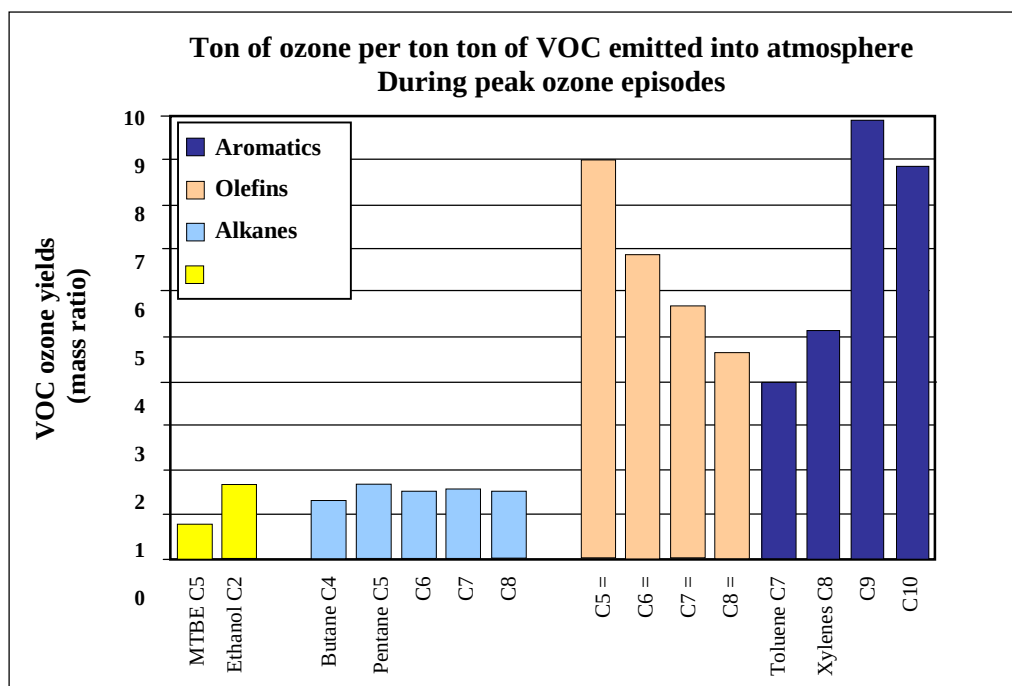
Figure 1.6. Ozone yields of individual petrol VOCs in the atmosphere
