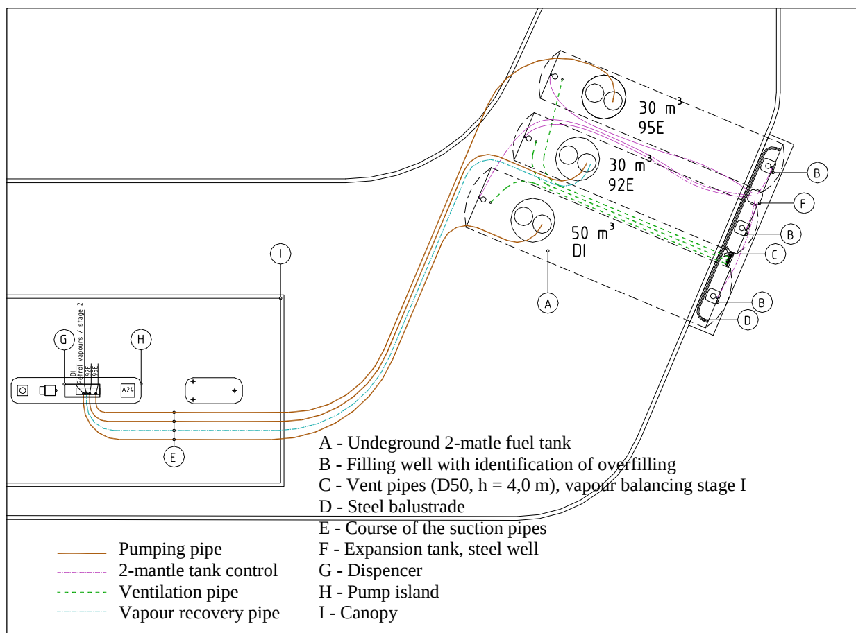
Figure 1.11. Typical petrol filling station's technology layout
