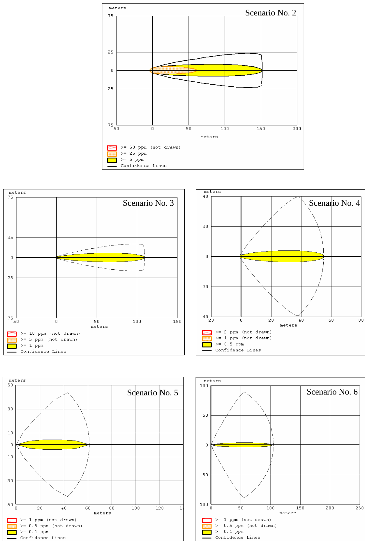
Figure 4.2. Modelled ethylbenzene toxic threat zone
