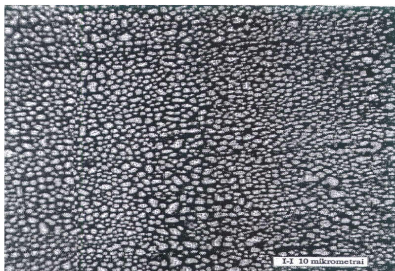
Fig. 2.11 Micropicture (x100) of heavy fuel oil-glycerol emulsion structure after 3 months storage and mechanical activation
