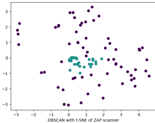
(a) t-SNE, perplexity=40 for ZAP scanner
