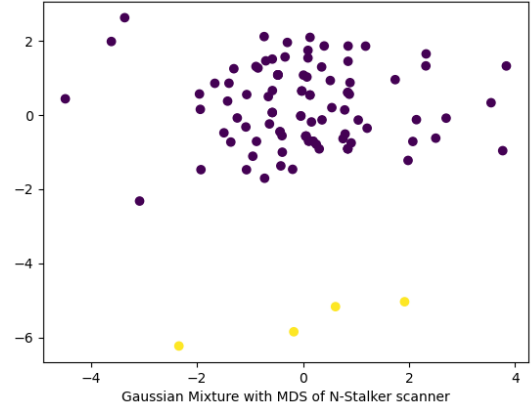
(b) gm=2, metric = 'False'
