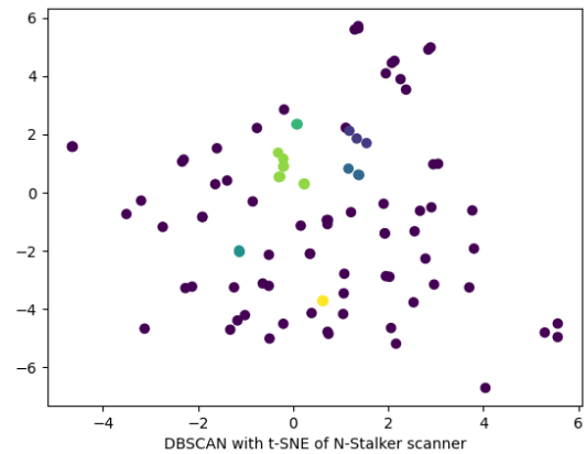
(b) t-SNE, perplexity=40 for N-Stalker scanner
