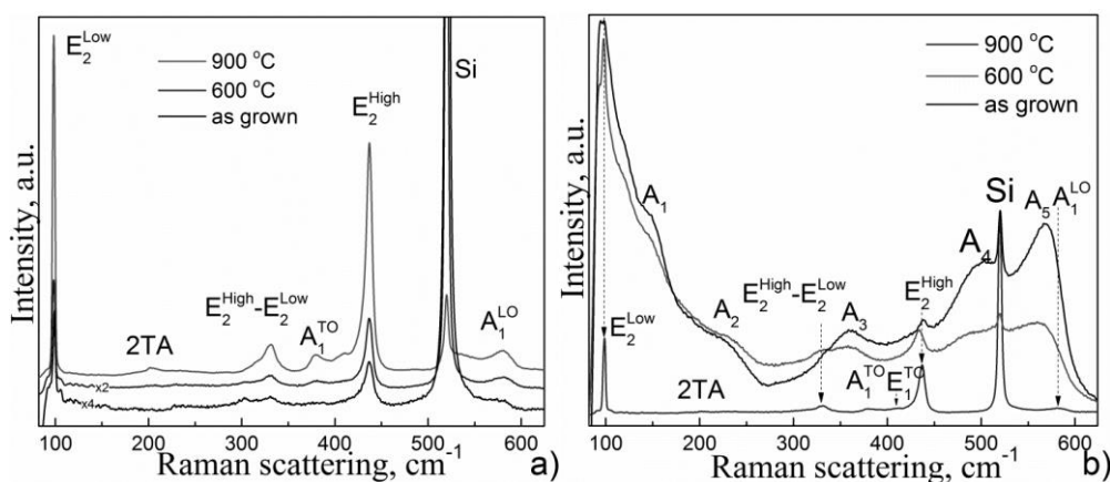
Fig 2. Raman scattering spectra of as-grown and annealed ZnO NS deposited on Si (a) and Ag/Si (b) substrates by APMOCVD.
