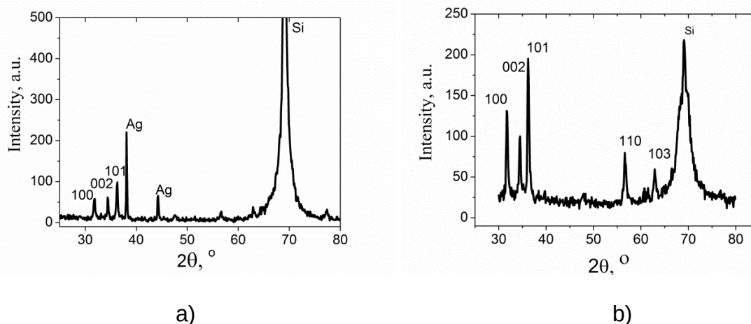
Fig.1 XRD patterns of ZnO NS deposited on Si (a) and Ag/Si (b) substrates by APMOCVD.
