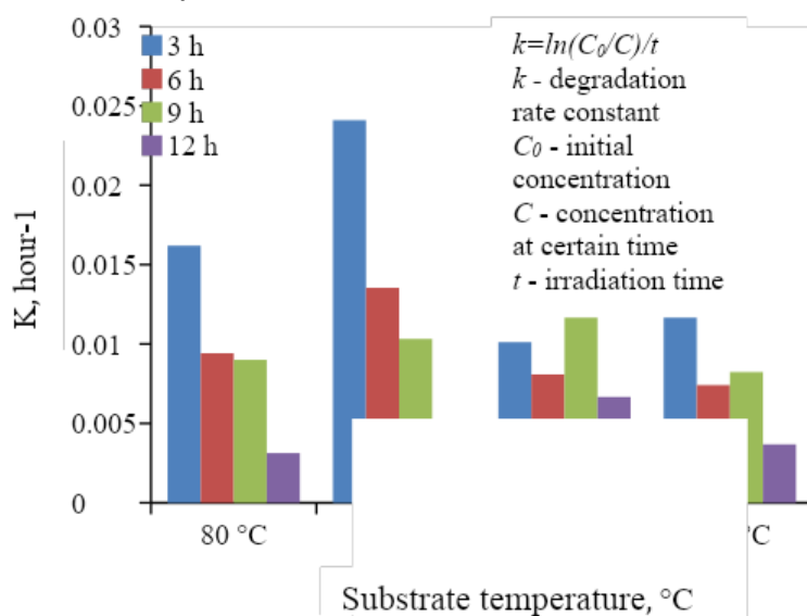
Fig. 2 Degradation rate constants of MO in the presence of \text{CuAl}_2\text{O}_4 films under UV irradiation
