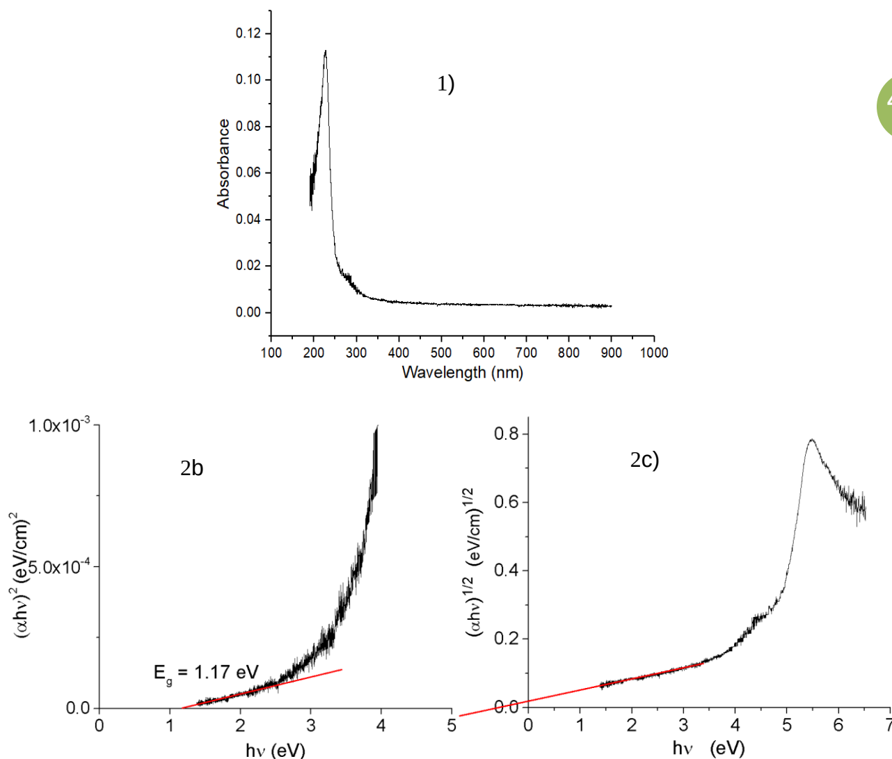
Fig. 1. (1) Ultraviolet-visible absorption spectrum of triple layer graphene nanostripes dispersed in isopropanol; (2) Tauc's plot derived from the absorption spectrum for the estimation of the graphene band-gap (2b) direct and (2c) indirect transition ( E_g = 1.1798 eV).
