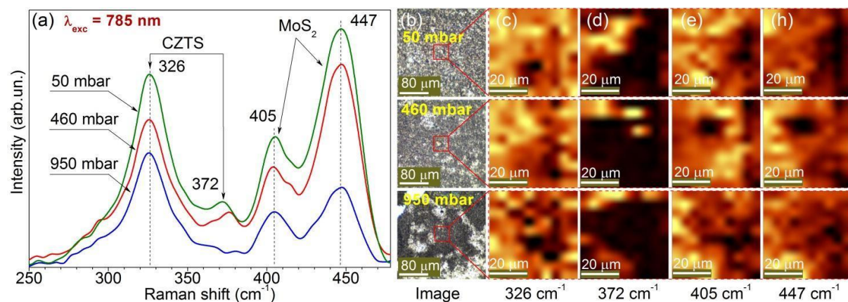
Fig. 1. \mu -Raman spectra (785 nm excitation) of the CZTS samples sulfurized at different P_{Ar} (a); their optical images (column b); and confocal Raman mapping over areas of 45 × 45 μm 2 with resolution of 4.5 μm for the bands at 326 (c), 372 (d), 405 (e), and 447 cm -1 (h).
