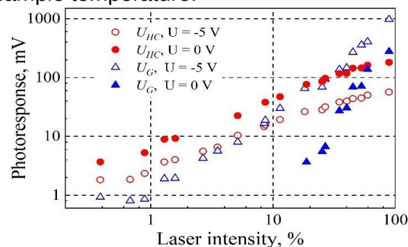
Fig. 1. Dependence of U_{HC} and U_G components on relative laser intensity at different bias voltage values.
