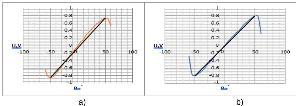
Fig 1. Dependence of differential voltage of working channels of photocells on the angle of inclination of light radiation: a) - sensor mounted on the satellite "Polyitan-2", b) - for the modified sensor.
