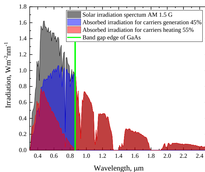
Fig.1 Absorption of solar spectrum AM 1.5 G by a GaAs solar cell.
