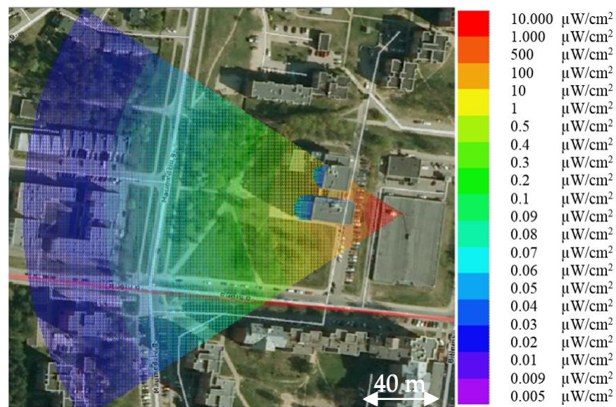
Figure 9. The dispersion of the electromagnetic radiation emitted by the antenna for mobile telecommunications KATHREIN 742241 through the area of 5 Rugiu str. in Vilnius (coordinates— 56^{\circ}20'32.7'' N, 23^{\circ}39'57.05'' E). Occupied area is 0.25 \text{ km}^2 .
