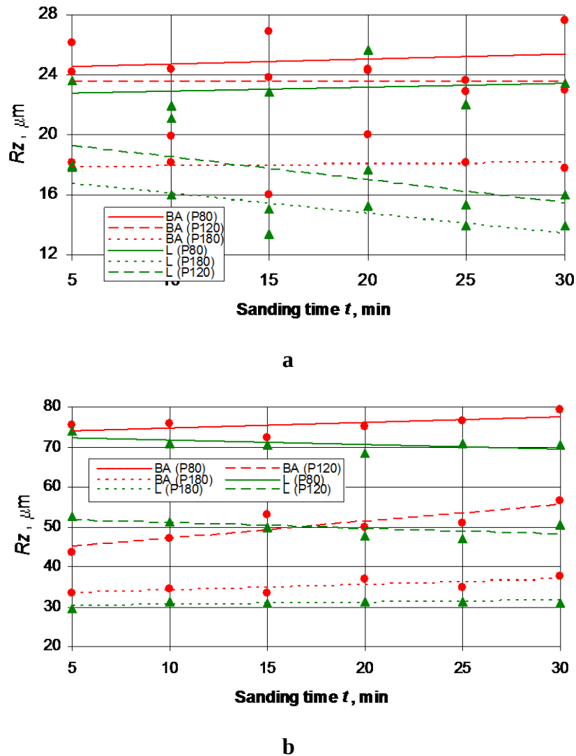
Figure 2. Surface roughness parameter R_z : a – along the grain; b – across the grain
