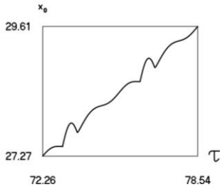
a) Displacement x_0 as function of \tau
