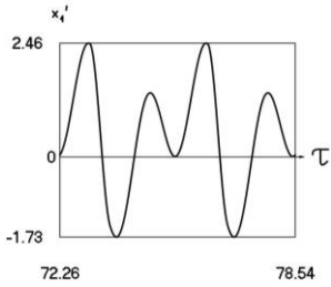
d) Velocity x'_1 as function of \tau
