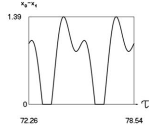
f) Difference of displacements x_0 - x_1 as function of \tau
