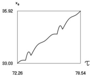
a) Displacement x_0 as function of \tau
