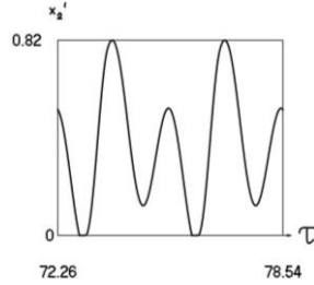
e) Velocity x'_2 as function of \tau
