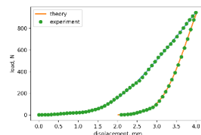
Figure 2: Load displacement relations.
