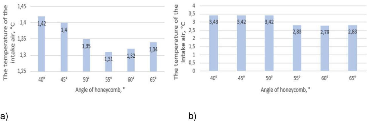
Fig. 2. The airflow temperature in the intake grill obtained for empty cabinet (a) and cabinet full of food products (b)
