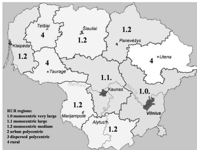
Fig. 2.11. RUR delineation and morphology classification for Lithuania (Nilsson et al. , 2013) demonstrates the peculiarities of the rural-urban interface in Lithuania. Map by the author
