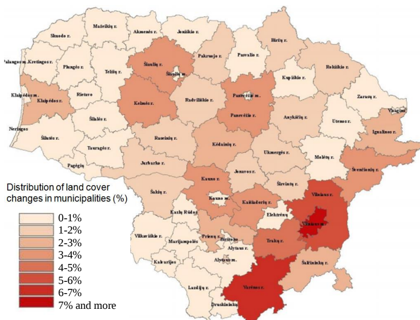
Fig. 1.5. Land cover changes 2006–2013 (Žemės..., 2014) in Lithuania demonstrating the constant landscape change and the urbanity as a driver in it (we should note the intensity of landscape change in the municipalities of Vilnius and Vilnius District).
