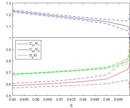
b: \rho = -0.7 .
