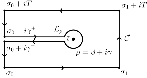
Figure 31: Contour \mathcal{C}' , with loop \mathcal{L}_\rho around the f zero \rho .
