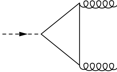
Figure 5: The Feynman diagram of the SM Higgs boson decay into a gluon-gluon pair.
