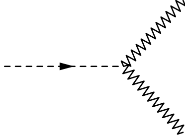
Figure 4: The Feynman diagram of the SM Higgs decay into EW bosons.
