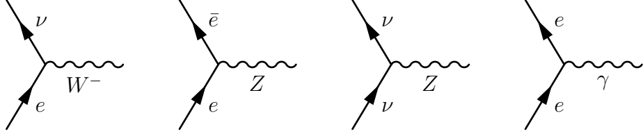
Figure 1: Interactions between leptons and vector bosons.
