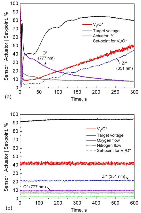
Fig. 11. Process control experiment in which the set-point for the V_T/\text{O}^* ratio is ramped from 10% (transition region near ‘fully poisoned’ mode) to over 50% (transition region near ‘metal’ zone) (a) and an example of process data from a deposition run where the V_T/\text{O}^* ratio is used for closed-loop gas flow control (b).
