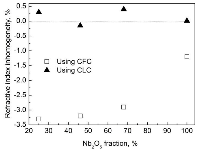
Fig. 17. Refractive index inhomogeneity of \text{Nb}_2\text{O}_5/\text{SiO}_2 mixtures deposited with constant \text{O}_2 flow and with closed-loop control.
