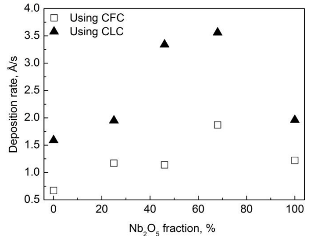
Fig. 15. The deposition rates of pure oxide materials ( \text{Nb}_2\text{O}_5 , \text{SiO}_2 ) and their mixtures deposited using two different reactive sputtering process control methods.
