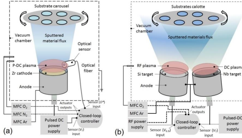
Fig. 2. Schematic diagram showing the process chamber used for: (a) \text{ZrO}_2 films deposition, (b) \text{Nb}_2\text{O}_5/\text{SiO}_2 mixture thin films.
