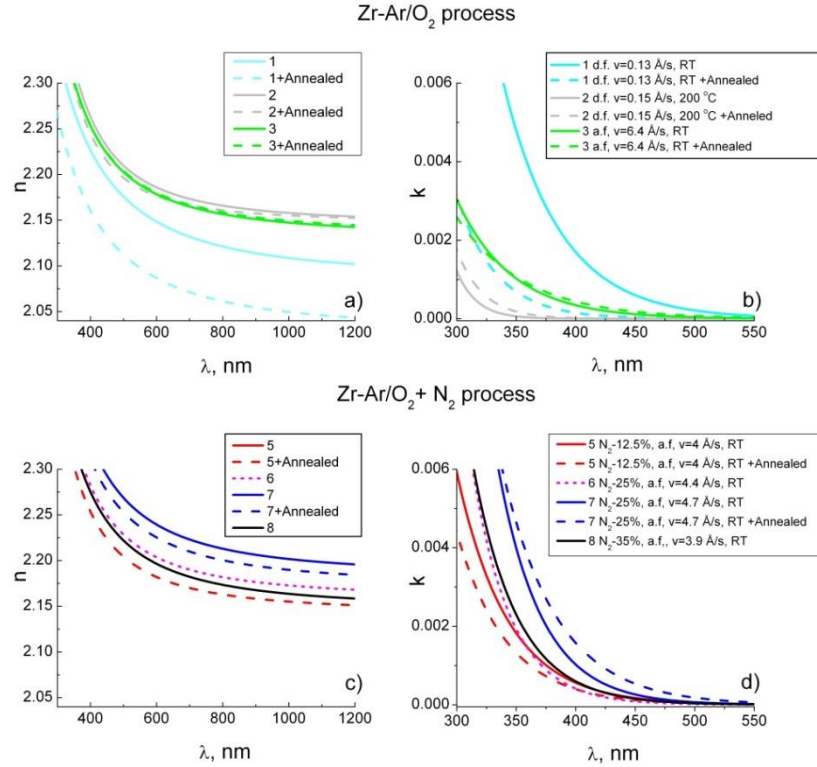
Fig. 13. Refractive index and extinction coefficient dispersions of \text{ZrO}_2 films deposited by reactive sputtering with and without active feedback process control.
