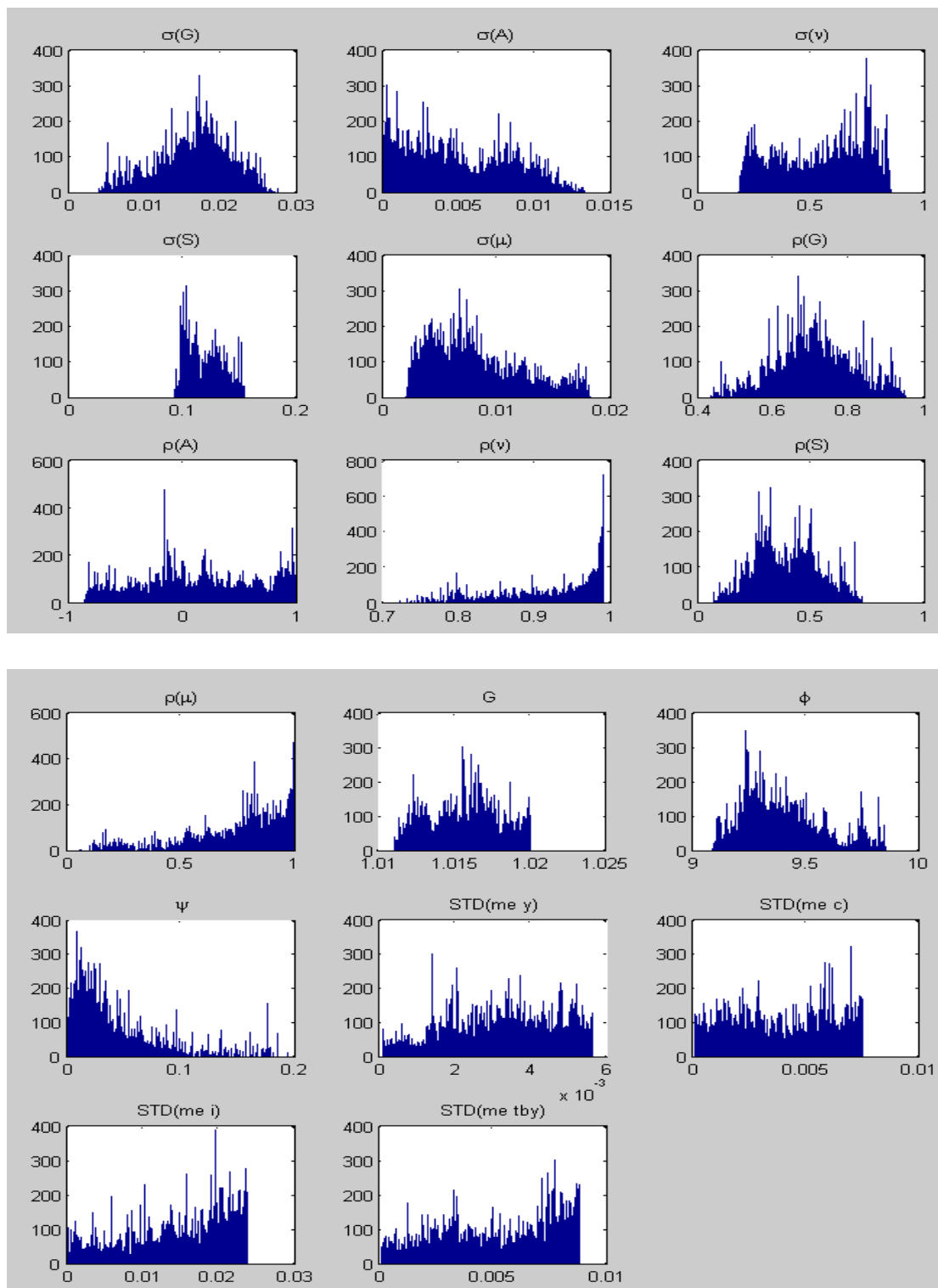
Figure 17. Estimated posterior distributions of the model parameters
