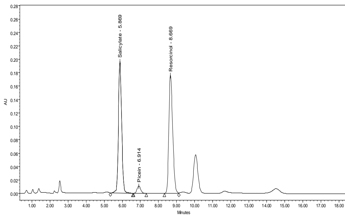
Fig. 2. Chromatogram obtained from test solution of Salix purpurea cl. 04132
