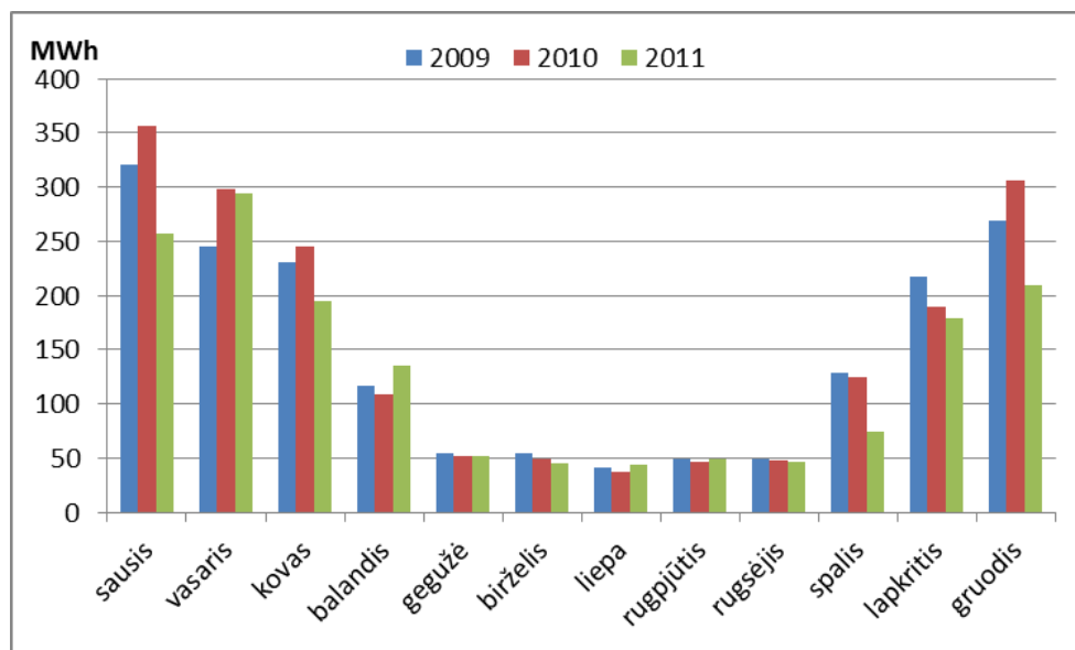
Heat consumption in Gargždai boiler No. 6 in 2009–2011, MWh
